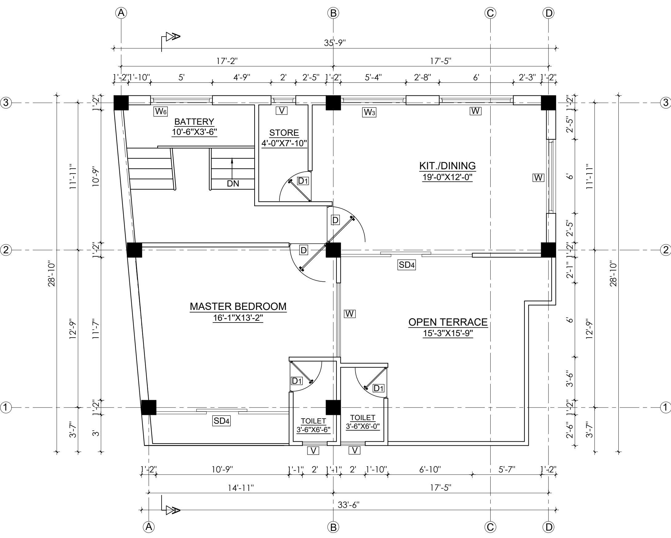
TOP FLOOR PLAN AREA=708.13 SQ.FT.
